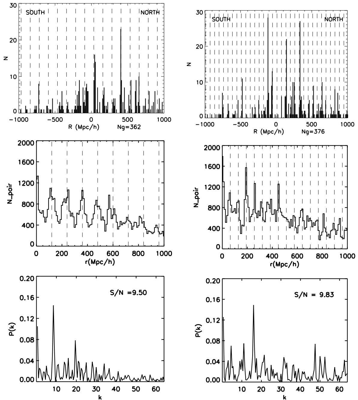
Figure 6. Selected samples (a)–(f). Plotted as for Fig. 5.
