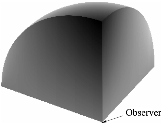
Figure 1. The shape of a light-cone and the observer point. The radius of the sphere is 1500 h^{-1} in both the \tau CDM and the \Lambda CDM models.
