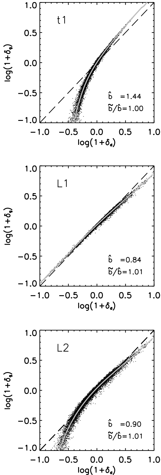
Figure 4. The joint distribution of the overdensity fields of ‘galaxies’ and mass, both smoothed with a 8h^{-1}\text{Mpc} top-hat window. The grey lines show the mean biasing function b(\delta) . Dashed lines show a linear relation \delta_g = \delta_s for a reference. The measured biasing parameters \hat{b} and \tilde{b}/\hat{b} are given in each panel.
