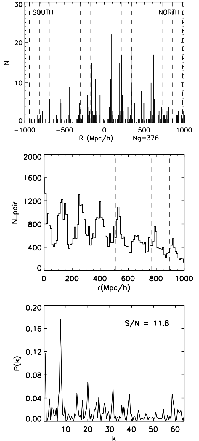
Figure 5. The BEKS data. Plotted are the distance histogram of galaxies (top), the pairwise separation histogram (middle), and the power spectrum (bottom). The height of the highest peak in the power spectrum and the values of \Delta and R (see text) are given to the top of the distant histogram.
