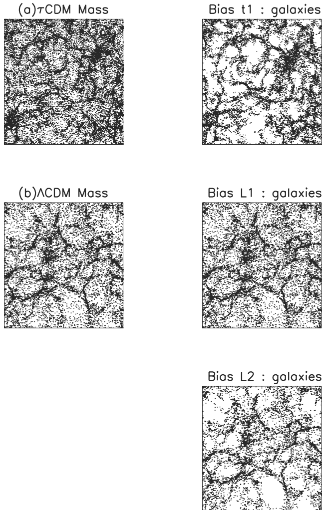
Figure 3. The distribution of the simulation dark-matter particles (left panels) and the biased ‘galaxies’ (right panels) in real space. The panels show 200 \times 200 \times 10 h^{-3} \text{Mpc}^3 slabs. Note the difference in the number density of the simulation dark-matter particles between the \tau CDM model ( 0.125 h^3 \text{Mpc}^{-3} ) and the \Lambda CDM model ( 0.037 h^3 \text{Mpc}^{-3} ). Strong bias effects are apparent in t1 and L2, whereas in L1 essentially no bias is seen.
