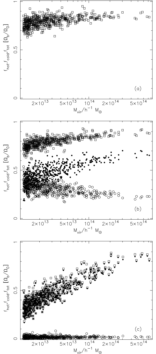
Figure 3. Mass fractions of hot gas (solid circles), cold gas (open circles) and the total fractions (squares) within the virial radius of clusters in the (a) Non-radiative , (b) Radiative and (c) Preheating simulations.
