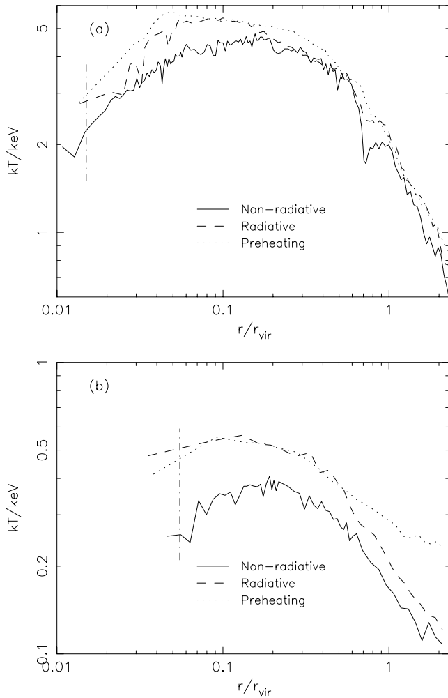
Figure 6. The mass-weighted temperature profiles of (a) the third most-massive and (b) the 10 least-massive clusters that did not show significant substructure. The long dash-dotted line indicates the gravitational softening length. Bins were chosen so as to average over at least 32 particles near the cluster core, with more further out.
