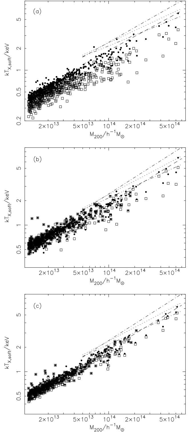
Figure 10. The X-ray temperature versus mass relation for the (a) Non-radiative , (b) Radiative and (c) Preheating simulations. The open squares show the total soft-band X-ray temperature, whereas the filled circles exclude emission from (a) gas with short cooling times, or (b,c) gas within the cooling radius. The different lines are from observations (Horner et al. 1999) using mass estimates from galaxy velocity dispersions (dashed line), X-ray temperature profiles (dot-dashed line), the isothermal- \beta model (dotted line), and emissivity profiles derived by surface brightness deprojection (triple-dot-dashed line).
