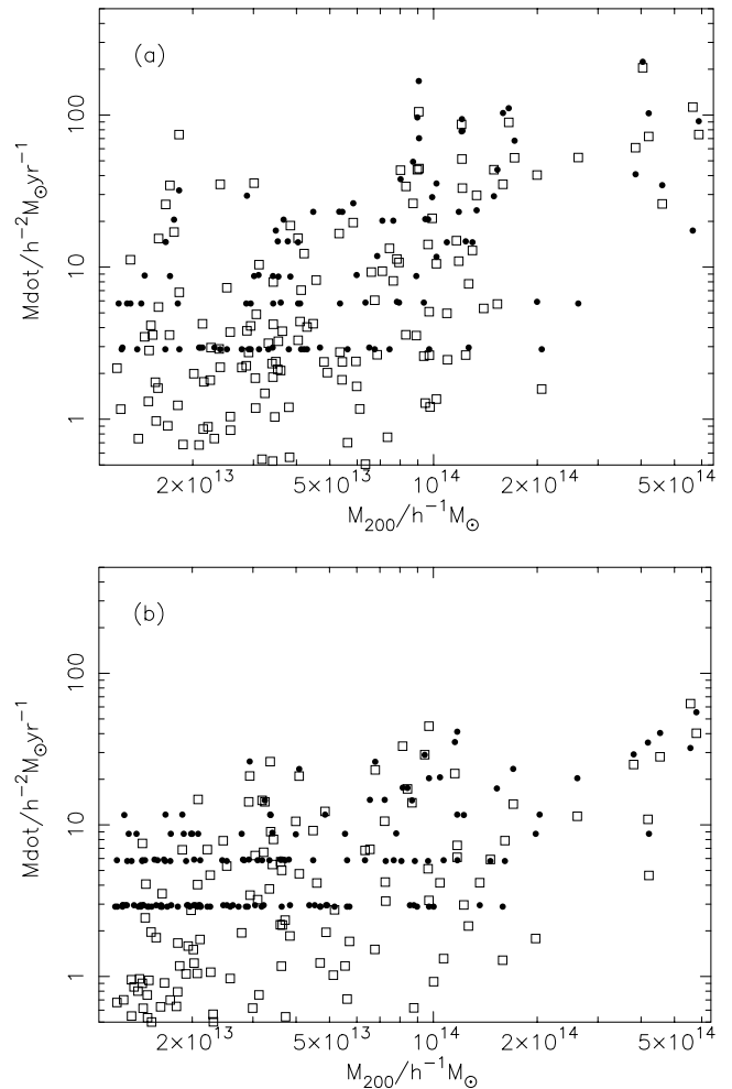
Figure 9. The mass deposition rates for clusters drawn from the (a) Radiative and (b) Preheating simulations. The open squares show the predicted mass deposition rate based on the soft-band X-ray emission from within the cooling radius; the solid circles show the actual mass deposition rate averaged over approximately 1 Gyr.
