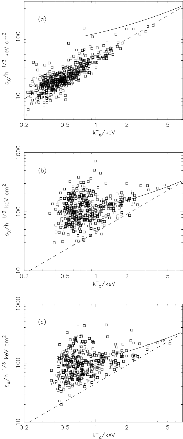
Figure 4. Core entropy at 0.1r_{\text{vir}} versus X-ray temperature for clusters in the (a) Non-radiative , (b) Radiative , and (c) Preheating simulations. The straight dashed line is the self-similar relationship from the simulations of Eke et al. (1998). The solid curve is an approximate fit to the Ponman et al. (1999) data points from their fig. 2.
