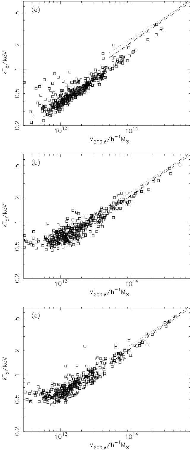
Figure 11. The X-ray temperature versus mass relation for the (a) Non-radiative , (b) Radiative and (c) Preheating simulations, where the mass is estimated from the isothermal- \beta model. The dotted, dashed and dot-dashed lines are observed masses using isothermal- \beta model from HMS99, FRB01 and XJW01, respectively.
