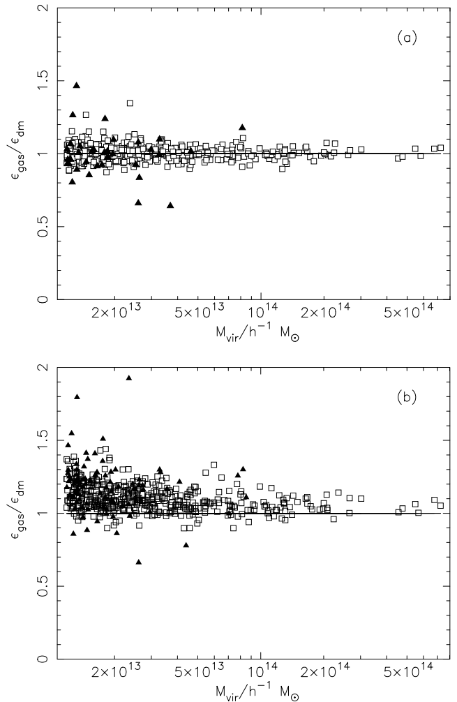
Figure 1. Ratios between the specific energy of the gas and the dark matter within the virial radii of clusters in the (a) Non-radiative and (b) Radiative simulations. The filled triangles correspond to clusters that show significant velocity substructure, as described in the text.
