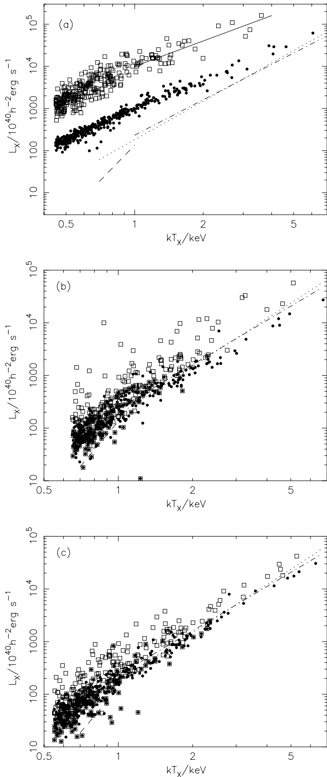
Figure 12. The bolometric X-ray luminosity versus temperature as estimated from the soft band for the (a) Non-radiative , (b) Radiative and (c) Preheating simulations. The open squares use the total soft-band emission, whereas the filled circles exclude emission from (a) gas with short cooling times, or (b, c) gas within the cooling radius. The dashed, dot-dashed and dotted lines are observed relations from Xue & Wu (2000); the solid line in panel (a) shows the self-similar relation L_X \propto T_X^2 .
