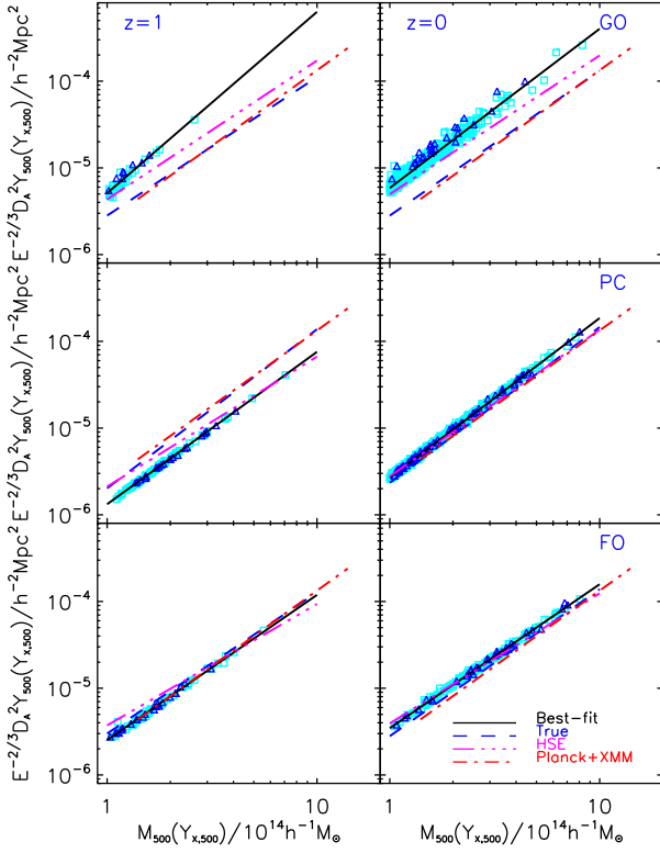
Figure 21. Y_{500} - M_{500} relations for the three models at z = 1 and z = 0 when r_{500}/M_{500} is estimated from the best-fit M_{500}^{\text{HSE}} - Y_{X,500}^{\text{HSE}} relation with no scatter. We also show the best-fit true Y_{500} - M_{500} relation (dashed line), the best-fit Y_{500}^{\text{HSE}} - M_{500}^{\text{HSE}} relation (triple-dot-dashed line) and the best-fit z < 0.5 relation from PXMM data (Planck Collaboration 2011c; dot-dashed line). The PC and FO models agree well with the observational data although there is a slight offset. The scatter is much lower, however, due to the strong correlation between Y_{500} and Y_{X,500} .
