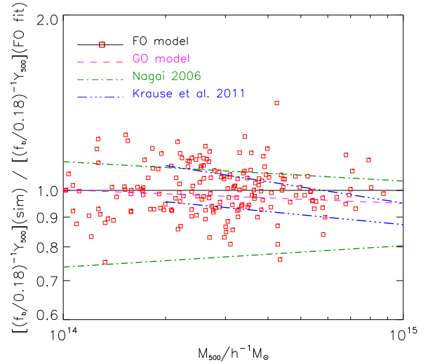
Figure 14. Comparison between the FO Y_{500} - M_{500} scaling relation and results from other simulations at z = 0 . All results are normalised to the best-fit FO Y_{500} - M_{500} relation and Y_{500} values from other simulations have been re-scaled to account for differences in baryon fraction (see text for details). The square symbols are individual cluster Y_{500} values from the FO model and the dashed line the best-fit GO relation. The dot-dashed lines are best-fit relations from Nagai (2006); the upper line corresponds to their non-radiative (AD) simulation and the lower line their run with cooling and star formation (CSF). Finally, the triple-dot-dashed lines are taken from Krause et al. (2011) for their restricted A and B samples (upper and lower lines respectively).
