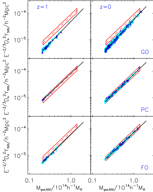
Figure 11. Scaling relations between Y_{500} and hot gas mass, M_{\text{gas},500} for the GO, PC and FO models at z = 1 and z = 0 . Details for each panel are the same as described in Fig. 8. The scatter is particularly small for the simulated version of this relation as the quantities plotted on the two axes are strongly correlated.
