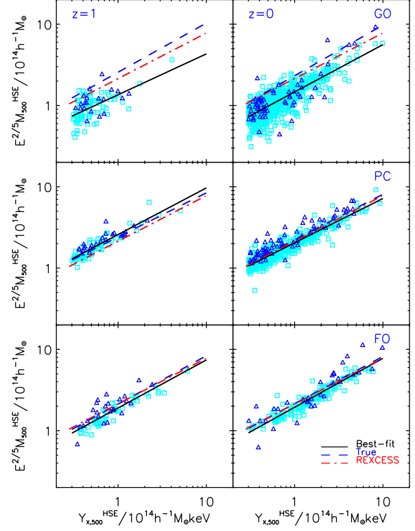
Figure 20. As in Fig. 19 but for the M_{500}^{\text{HSE}} - Y_{X,500}^{\text{HSE}} relation. Clusters are now selected with 3 \times 10^{13} < Y_{X,500}^{\text{HSE}} < 10^{15} which, for the PC and FO models, matches well to our normal mass range. The solid line is the best-fit to the relation and the dashed line the true relation. The dot-dashed line is the best-fit relation from REXCESS ( XMM-Newton ) data as found by Arnaud et al. (2010).
