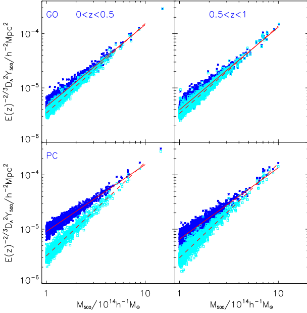
Figure 15. Projected Y_{500} - M_{500} relations for clusters in the GO (top panels) and PC (bottom panels) sky maps with 0 < z < 0.5 (left panels) and 0.5 < z < 1 (right panels). The stars correspond to Y_{500}^{\text{sky}} values, i.e. calculated from the full sky map. The squares correspond to Y_{500}^{\text{clus}} values, i.e. from the cluster region. In both cases the true M_{500} values were used. The dashed line is a best-fit to the Y_{500}^{\text{clus}} - M_{500} relation and the solid line to the Y_{500}^{\text{sky}} - M_{500} relation. The Y_{500}^{\text{sky}} values are higher on average than Y_{500}^{\text{clus}} , especially in the PC simulation at low mass and low redshift, where the difference is a factor of 2-3.
