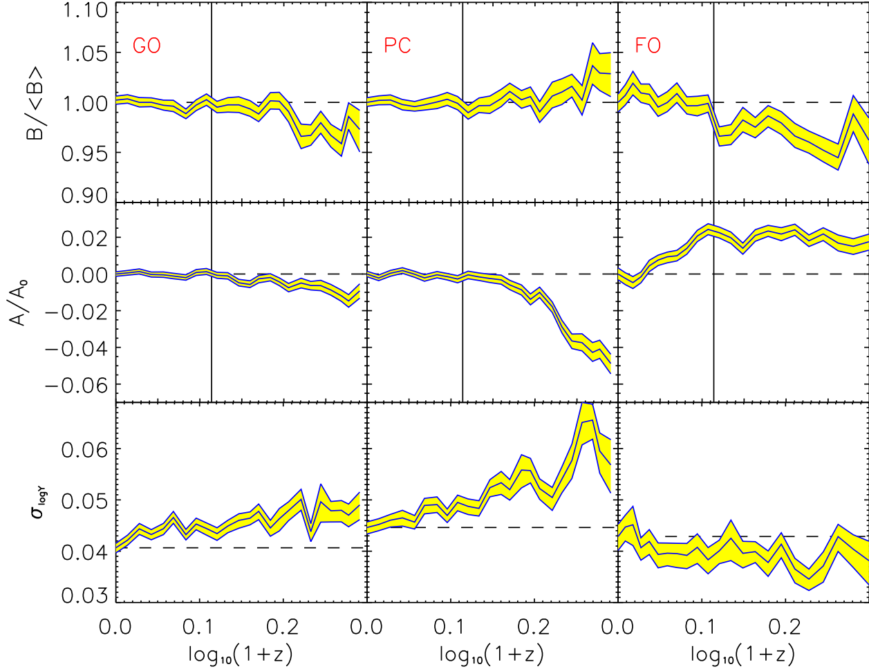
Figure 10. The dependence of the slope, normalisation and scatter of the E(z)^{-2/3}Y_{500} - M_{500} relation with redshift, for the GO (left), PC (middle) and FO (right) simulations. Results are plotted from z = 0 to z = 1 . In the top panels, the best-fit slope at each redshift is normalised to the median slope for outputs at z < 0.3 (shown as a vertical line). The middle panels illustrate the redshift dependence of the normalisation after the self-similar dependence has been taken out; the normalisation is divided by the z = 0 value in this case. In the bottom panels, the rms scatter in \log_{10} Y , \sigma_{\log_{10} Y} , is shown as a function of redshift. For both the normalisation and scatter values, the slope was fixed to the z < 0.3 median value when performing the fits. The bands in all panels illustrate 16 and 84 per centiles, calculated by bootstrap resampling the data. All three models predict very little evolution in the slope and normalisation of the E(z)^{-2/3}Y_{500} - M_{500} relation to z = 1 and the intrinsic scatter remains small ( \sigma_{\log_{10} Y} < 0.06 ).
