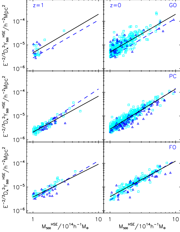
Figure 19. The Y_{500}^{\text{HSE}} - M_{500}^{\text{HSE}} relations (i.e. using estimated values for each cluster assuming the gas is hydrostatic) for the GO, PC and FO models at z = 1 and z = 0 . The squares correspond to regular clusters while the triangles are disturbed clusters. The solid line is the best-fit relation while the dashed line shows the best-fit true Y_{500} - M_{500} relation. Fits are performed for all clusters with 10^{14} h^{-1} M_{\odot} < M_{500}^{\text{HSE}} < 10^{15} h^{-1} M_{\odot} and best-fit parameter values are given in Table 5. It is clear that the hydrostatic assumption is more robust for the PC and FO runs than for the GO run.
