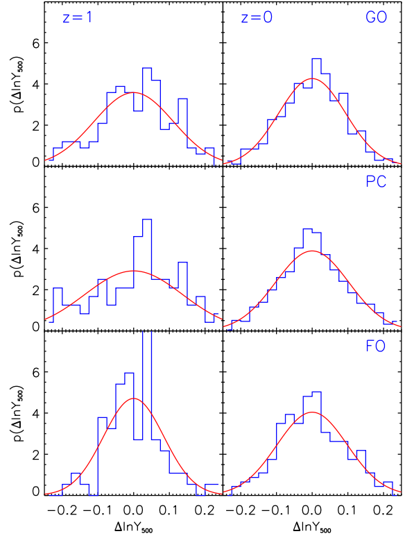
Figure 9. Distribution of residual Y_{500} values about the best-fit Y_{500} - M_{500} relation, plotted using natural logarithms, for each of the models at z = 1 and z = 0 . A normal distribution of width \sigma = \sigma_{\ln Y} is overlaid; it is clear that this provides a good description of the scatter.
