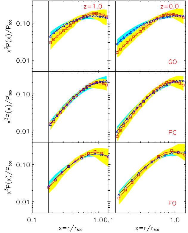
Figure 5. As in Fig. 4 but the samples are now split into regular ( s \leq 0.1 ; triangles) and disturbed ( s > 0.1 ; squares) sub-samples. Disturbed (merging) clusters tend to have lower central pressures but higher peak values of x^3 P(x) .
