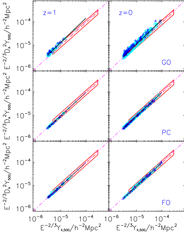
Figure 13. Scaling relations between the SZ Y_{500} and the X-ray analogue, Y_{X,500} . Details for each panel are the same as described in Fig. 8. The dot-dashed line corresponds to Y_{500} = Y_{X,500} ; only the GO simulation shows a significant offset from this relation, due to the presence of clumpy low-entropy gas.
