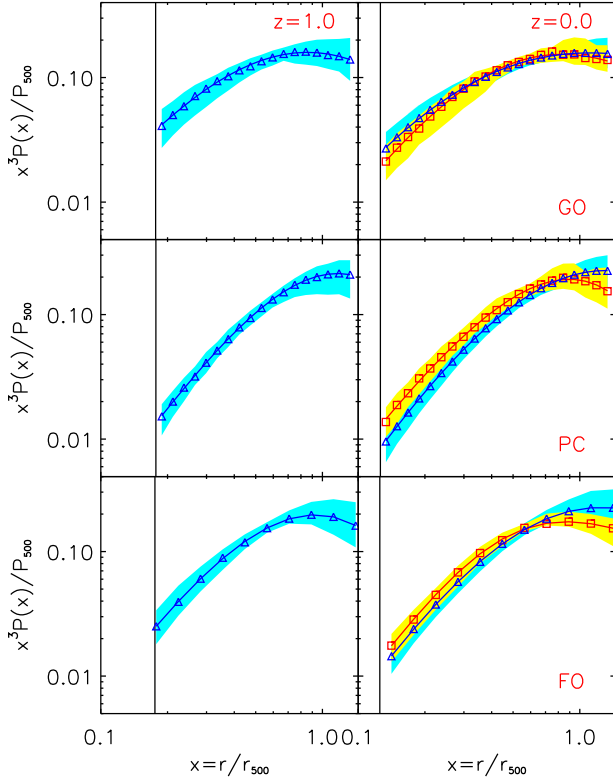
Figure 4. Scaled pressure profiles for clusters within the GO (top panels), PC (middle panels) and FO (bottom panels) simulations. Left panels are z = 1 results and right panels for z = 0 . Median profiles are shown separately for low-mass ( 10^{14} h^{-1} M_{\odot} < M_{500} \leq 5 \times 10^{14} h^{-1} M_{\odot} ; triangles) and high-mass ( M_{500} > 5 \times 10^{14} h^{-1} M_{\odot} ; squares) respectively (note there are no high mass clusters at z = 1 ). The yellow (cyan) shaded band illustrates the 16/84 per centiles (and thus represents the cluster-to-cluster scatter) for the high-mass (low-mass) sub-sample. Solid curves are best-fit generalised NFW profiles to the median pressure profiles. The vertical solid line represents the radius where gravity is softened in the cluster with the smallest r_{500} (this is at a smaller radius than plotted for the FO model, for which a smaller softening was used, but we choose to use the same scale as in the other two models for ease of comparison). Note that the contribution to Y_{500} is predominantly from r > 0.5r_{500} and so is not particularly susceptible to variations in the cluster core.
