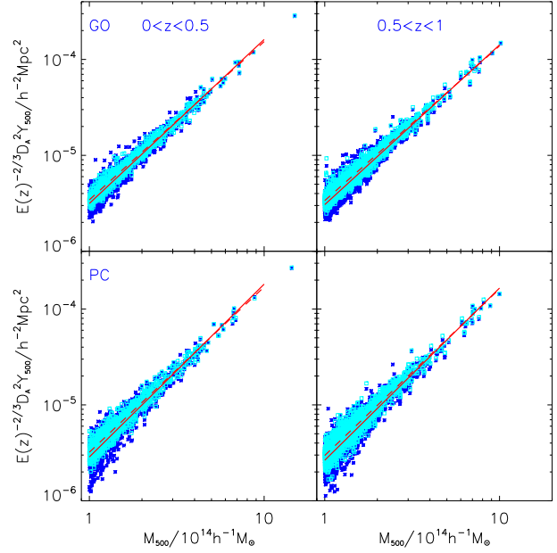
Figure 16. As in Fig. 15 but the Y_{500}^{\text{sky}} values have had the mean background signal subtracted. The two best-fit relations are now very similar in all panels.
