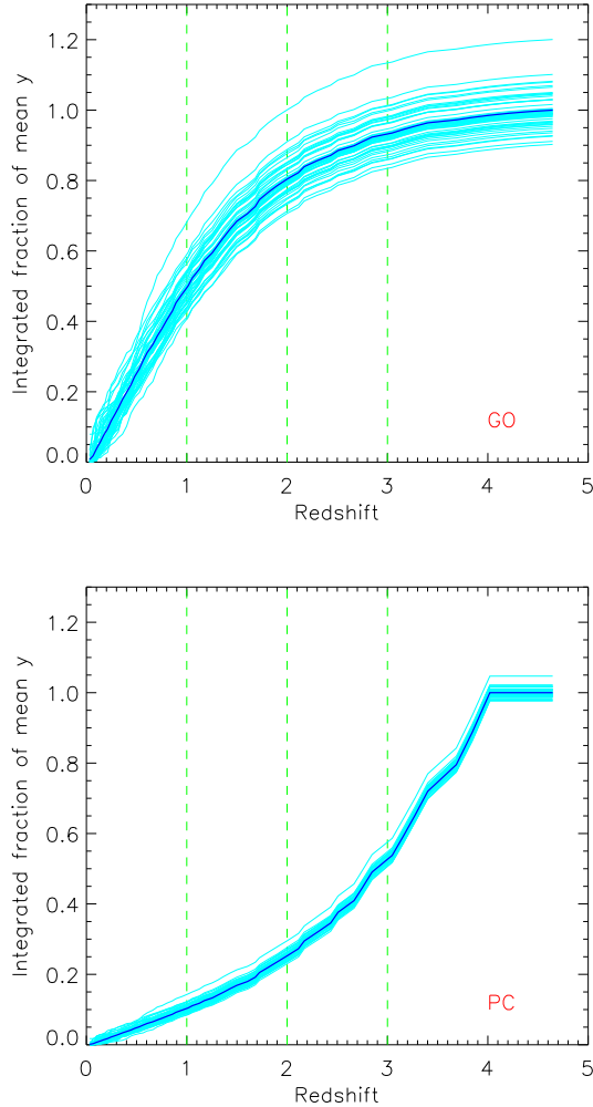
Figure 3. Integrated contribution to the overall mean y signal from gas below a given redshift. The top panel is for the GO simulation and the bottom panel for the PC simulation. Light curves are for individual maps and the dark curve is the average over all 50 maps. Each curve is normalised to the mean y averaged over all 50 maps, highlighting the scatter in the integrated signal between realisations. The simulations predict dramatically different redshift dependencies: the mean signal in the GO simulation comes from low redshift ( z < 2 ) whereas the opposite is the case for the PC simulation, due to the effect of pre-heating at z = 4 .
