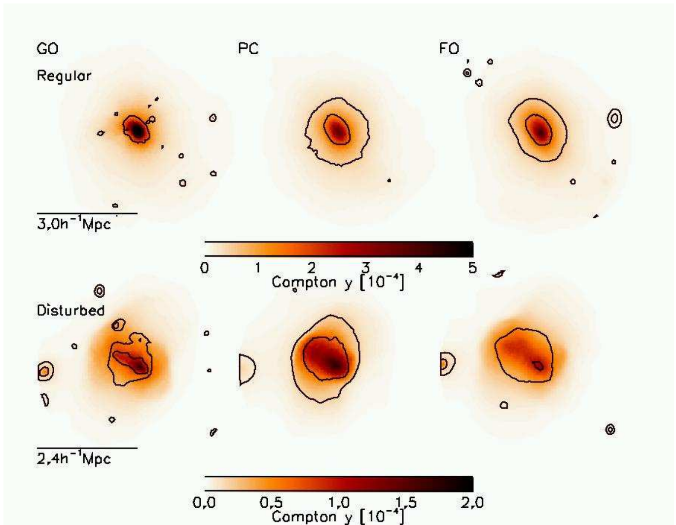
Figure 1. Top panels: Compton- y maps for the most massive cluster at z = 0 in the MS ( M_{\text{vir}} \simeq 2.9 \times 10^{15} h^{-1} M_{\odot} , which we classify as regular) with X-ray surface brightness contours overlaid. Results are shown, from left to right, for the cluster in the GO, PC and FO models respectively. Images in the bottom panels are similar except a massive disturbed cluster (with M_{\text{vir}} \simeq 1.5 \times 10^{15} h^{-1} M_{\odot} ) is shown. Each panel is 2r_{\text{vir}} across and the scale and value of r_{\text{vir}} is shown in the left-hand panels. The range of y values is given for each cluster in the scale at the bottom of each row; note the disturbed cluster has a lower maximum value than the regular cluster. The X-ray contours illustrate levels that are 10 per cent and 1 per cent of the maximum value in the map. The gross features are similar in all 3 models for both clusters, although the X-ray maps reveal that the gas in the the PC clusters is the smoothest, while the GO clusters contain gas with the most small-scale structure.
