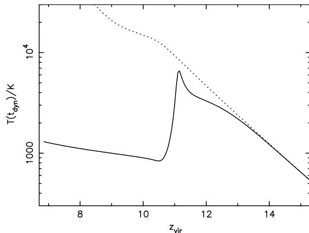
Figure 4. Temperature obtained after one dynamical time versus virialization redshift, for cosmology \tau CDM. The dotted line shows the initial, virial temperature of the halo. The cusp in the curve corresponds to a virial temperature of 9000 K.
