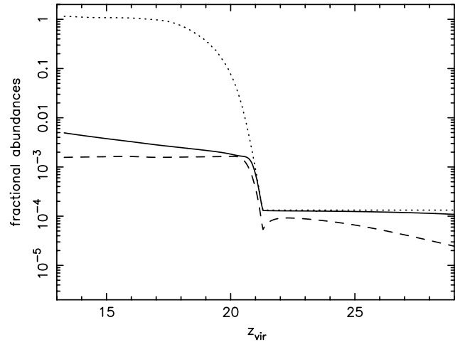
Figure 8. Ionization fraction (solid line) and \text{H}_2 abundance (dashed line) after one dynamical time, for cosmology \Lambda\text{CDM} . The dotted line shows the initial ionization level of the halo.
