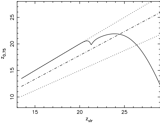
Figure 6. The solid line shows the redshift at which a gas halo will cool to 75 per cent of its initial temperature, z_{0.75} , versus virialization redshift, z_{\text{vir}} , for cosmology \Lambda\text{CDM} using the GP98 cooling function. The upper and lower dotted lines show the relations z_{0.75} = z_{\text{vir}} and z_{0.75} = 0.75z_{\text{vir}} , respectively; the dot-dashed line shows the redshift at one dynamical time after virialization.
