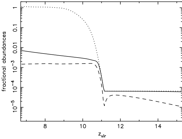
Figure 5. Ionization fraction (solid line) and \text{H}_2 abundance (dashed line) after one dynamical time, for cosmology \tau\text{CDM} . The dotted line shows the initial ionization level of the halo.
