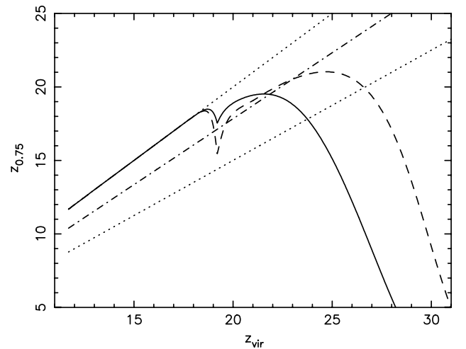
Figure 2. Redshift at which a gas halo will cool to 75 per cent of its initial temperature, z_{0.75} , versus virialization redshift, z_{\text{vir}} , for cosmology SCDM for two different cooling functions: dashed curve, LS84; solid curve, GP98. The upper and lower dotted lines show the relations z_{0.75} = z_{\text{vir}} and z_{0.75} = 0.75z_{\text{vir}} , respectively; the dot-dashed line shows the redshift at one dynamical time after virialization.
