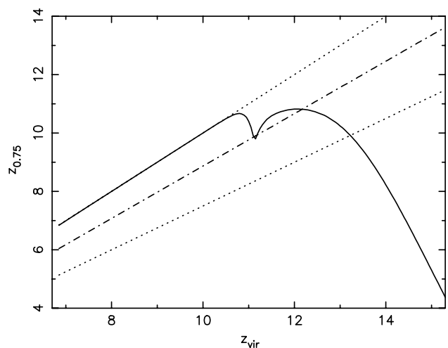
Figure 3. The solid line shows the redshift at which a gas halo will cool to 75 per cent of its initial temperature, z_{0.75} , versus virialization redshift, z_{\text{vir}} , for cosmology \tau CDM using the GP98 cooling function. The upper and lower dotted lines show the relations z_{0.75} = z_{\text{vir}} and z_{0.75} = 0.75z_{\text{vir}} , respectively; the dot-dashed line shows the redshift at one dynamical time after virialization.
