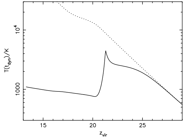
Figure 7. Temperature obtained after one dynamical time versus virialization redshift, for cosmology \Lambda\text{CDM} . The dotted line shows the initial, virial temperature of the halo.
