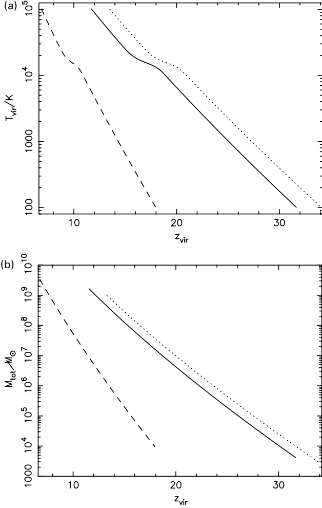
Figure 1. This figure shows the relation between virialization redshift and (a) temperature and (b) total mass for the three cosmologies: SCDM (solid line), \tau CDM (dashed line), and \Lambda CDM (dotted line).
