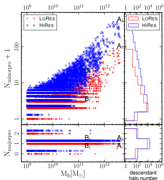
Figure 12. The number of progenitors a halo has as a function of its mass and histogram of the number of progenitors. The left lower panel counts the number of major progenitors, which have a mass larger than one third of their descendants', and the left upper panel counts the number of minor progenitors, which have a mass smaller than one third of their descendants'. Red pluses represent haloes from the LORES simulation and green crosses represent haloes from the HiRES simulation. The right lower panel represents the histogram of the number of major progenitors, and the right upper panel represents the histogram of the number of minor progenitors. Red lines indicate the LORES simulation and green lines indicate the HiRES simulation. All haloes from all snapshots with more than one progenitor are included. For clarity, points from the HiRES simulation are shifted up slightly.
