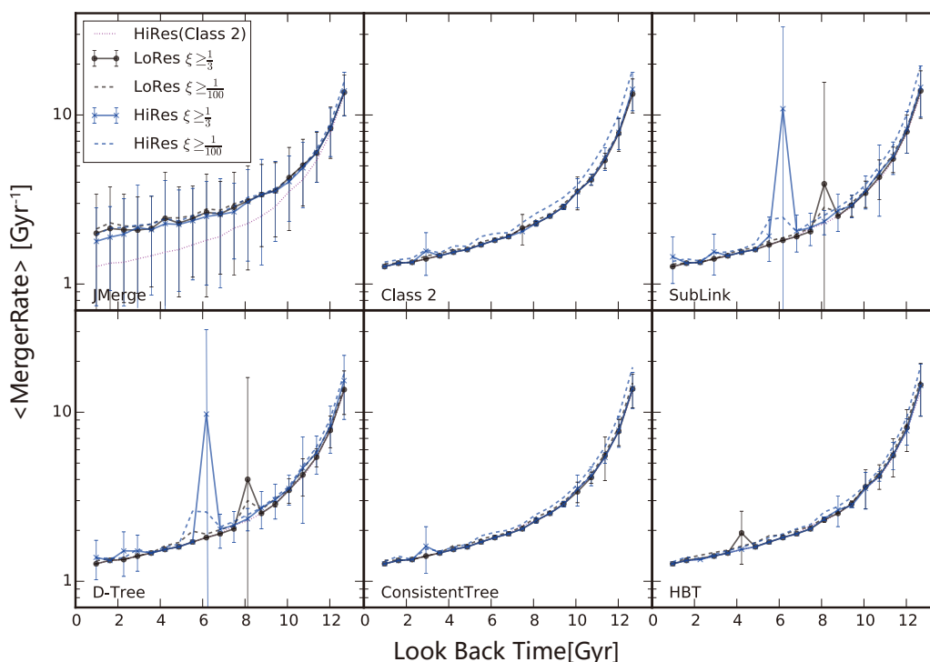
Figure 14. Mean merger rate (mergers per descendant halo per Gyr) as a function of look back time. Lines with different colour represent the merger trees built in the LORES and HIRES simulations, as shown by the legend. Solid lines show the merger rate with progenitor mass ratio larger than 1/3 . Dashed lines show the merger rate with progenitor mass ratio larger than 1/100 . The HIRES line of CLASS2 ( \xi \geq 1/3 ) is reproduced in magenta on all panels for guidance. The error bars show the rms in every time bin. Each subpanel displays results for one tree-builder as indicated, except for the four CLASS2 finders which are indistinguishable and so all shown on the same subpanel.
