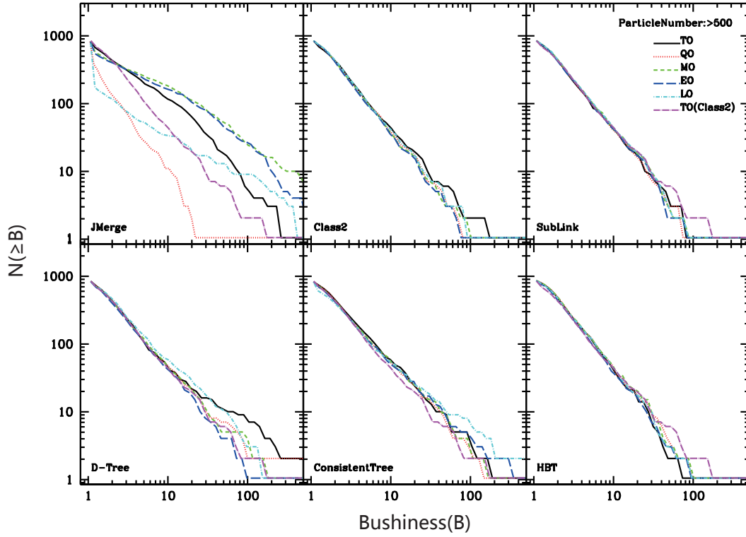
Figure 6. Merger tree bushiness B for each of the builders in SINGLEHALO simulation. Only root haloes with more than 500 particles are selected here. Each subpanel shows results for an individual tree-builder as indicated, except for the four class 2 finders which are indistinguishable and are therefore all shown on the same subpanel. Different line colours and styles represent different output strategies as indicated in the legend. The CLASS2 TO line is reproduced on all panels for guidance.
