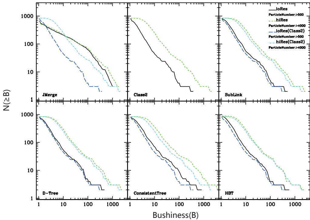
Figure 11. Number of trees of each bushiness B in the LORES and HiRES simulations. The criterion for selection and the linetypes are the same as for Figure 10
