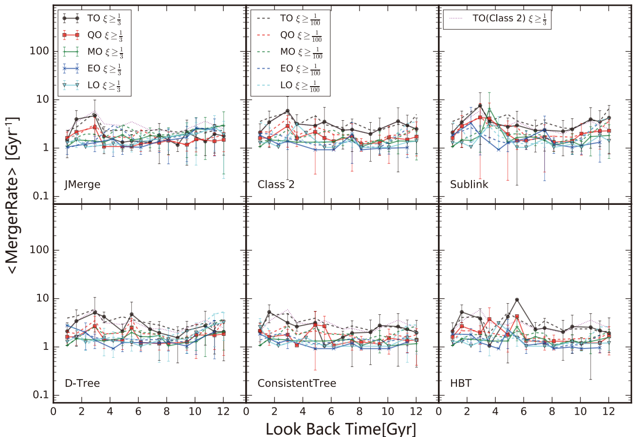
Figure 9. Mean merger rate (mergers per descendant halo per Gyr) as function of look-back time. Lines with different colour represent the merger tree built with a different output strategy, as shown by the legend. Solid lines show the merger rate with progenitor mass ratio larger than 1/3. Dashed lines show the merger rate with progenitor mass ratio larger than 1/100. The TO line of CLASS2 is reproduced in magenta on all panels for guidance. The error bars show the rms in every time bin. Each subpanel shows results for one tree builder as indicated, except for the four class 2 finders which are indistinguishable and so are all shown on the same subpanel.
