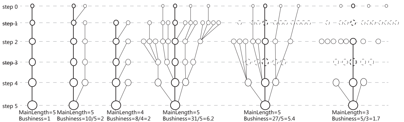
Figure 2. Calculation of main branch length L and bushiness B as defined in the text for 6 example trees. The thick line represents the main branch. If snapshots are dropped to form a smaller dataset then the fourth tree can become the fifth or the sixth depending on whether or not the progenitor branches are well linked. The sixth tree has a significantly reduced bushiness.
