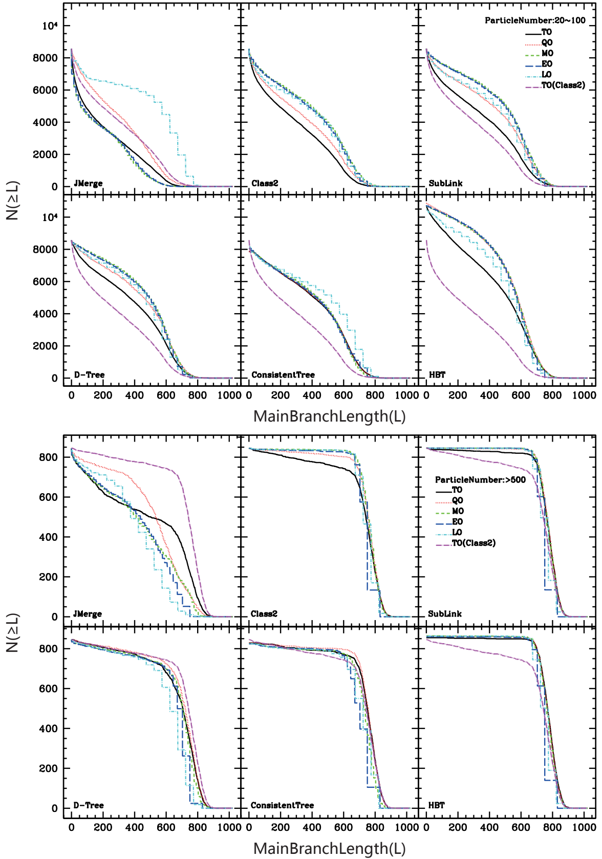
Figure 4. Cumulative number of merger trees with main branch lengths larger than L in the SINGLEHALO simulation. The upper panel with 6 subplots shows the results from merger trees with root haloes containing 20-100 particles, and the lower panel is for root haloes larger than 500 particles. Each subpanel shows the results of a tree-builder as labeled in the bottom left corner. Different line colours and styles represent different output strategies as indicated in the legend. The TO line of CLASS2 is reproduced in magenta on all panels for guidance.
