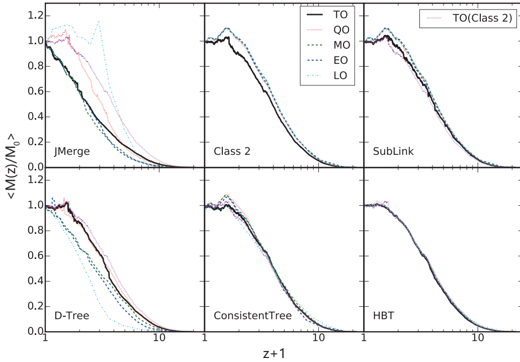
Figure 7. Average mass history for each of the builders as a function of redshift. This corresponds to the total mass in tree main branches for root haloes between 0.5 \times 10^9 M_\odot and 1.5 \times 10^9 M_\odot at z = 0 , normalized by the mass at z = 0 . Different lines represent merger trees built from different output strategies, as indicated by the legend. Each subpanel displays results for one tree builder as indicated, except for the four class 2 finders which are indistinguishable and so are all shown on the same subpanel. The TO line of CLASS2 is reproduced in magenta on all panels for guidance.
