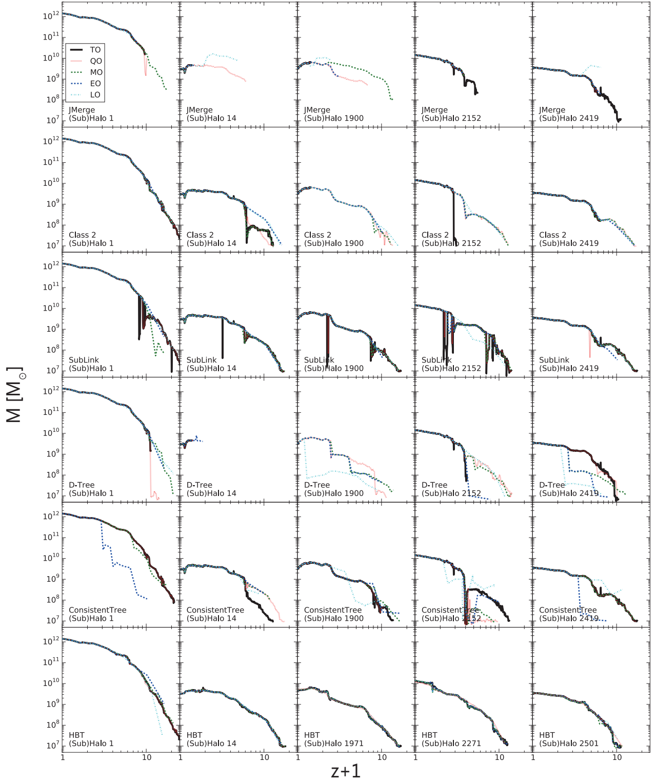
Figure 8. Mass histories for 5 (sub)haloes constructed by different merger-tree-builders. Different line styles represent different output strategies, as shown by the legend. Each row shows results for one tree builder as indicated, except for the four CLASS2 finders which are indistinguishable and so are all shown on the second row.
