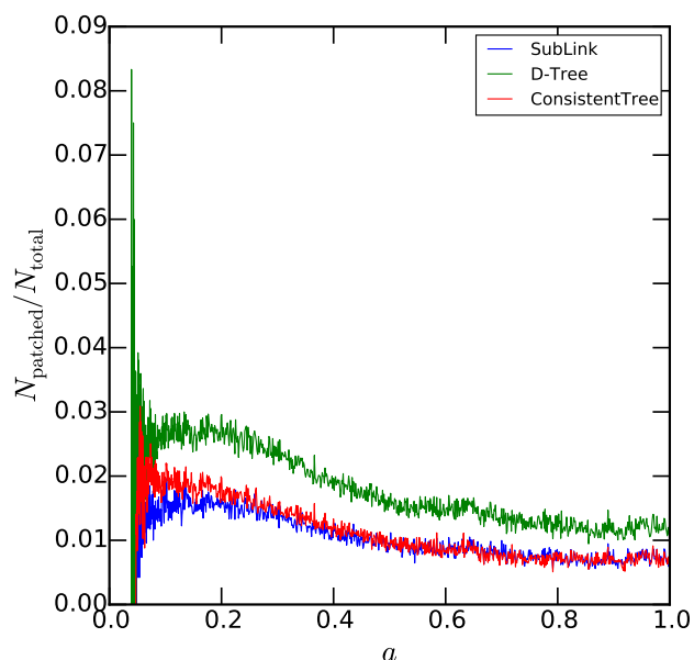
Figure 5. The fraction of patched haloes in every snapshot in the TO dataset as a function of the scale factor, a . Each line represents a different CLASS3 tree builder as indicated.
