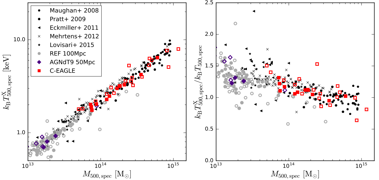
Figure 7. Spectroscopic temperature measured within r_{500, \text{spec}} as a function of estimated total mass at z = 0.1 for the C-EAGLE clusters and the REF and AGNdT9 groups and clusters. Marker styles are the same as in Fig. 2. The black pentagons, circles, left-facing triangles, crosses and stars show observational data from Maughan et al. (2008), Pratt et al. (2009), Eckmiller et al. (2011), Mehrtens et al. (2012) and Lovisari et al. (2015) respectively. The left panel shows the temperature and the right panel shows the temperature normalized by the virial temperature to approximately remove the mass dependence.
