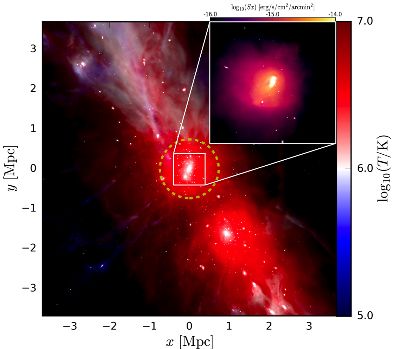
Figure 1. Image of CE-5 and its environment at z = 0.1 , resimulated using the EAGLE AGNt9 model. The colour map shows the gas, with the intensity depicting the density of the gas and the colour depicting the temperature of the gas. Stellar particles are shown by the white points and the dashed yellow circle denotes r_{200} . The inset colour map shows the X-ray surface brightness from a cubic region of 2r_{500} , centred on the cluster’s centre of potential.
