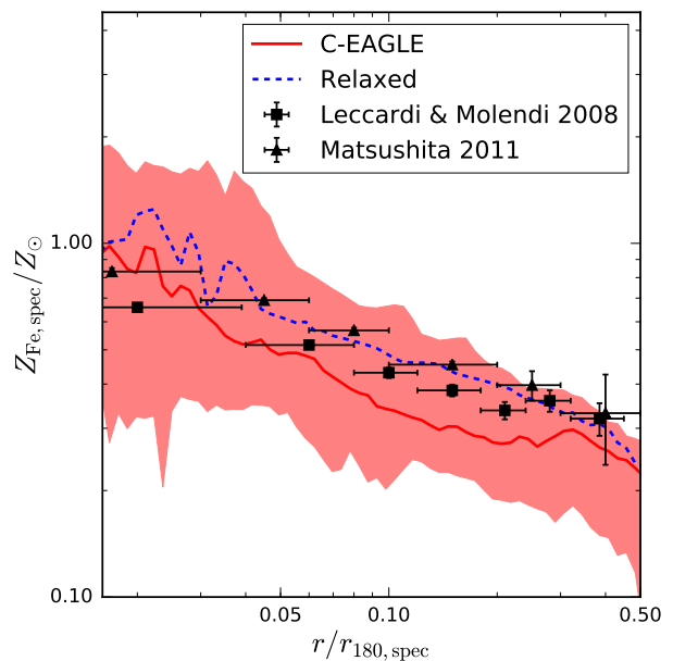
Figure 15. Median emission-weighted iron abundance profiles for the C-EAGLE sample and its relaxed subset at z = 0.1 . Marker styles are identical to Fig. 11. The black squares and triangles are the mean observed profiles from Leccardi & Molendi (2008) and Matsushita (2011), with the error bars showing the measurement uncertainty.
