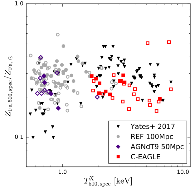
Figure 9. Mass-weighted iron abundance measured within r_{500,\text{spec}} as a function of spectroscopic temperature at z = 0.1 for the C-EAGLE clusters and the REF and AGNdT9 groups and clusters. Marker styles are the same as in Fig. 2. The black triangles show the homogenized observational data from Yates et al. (2017).
